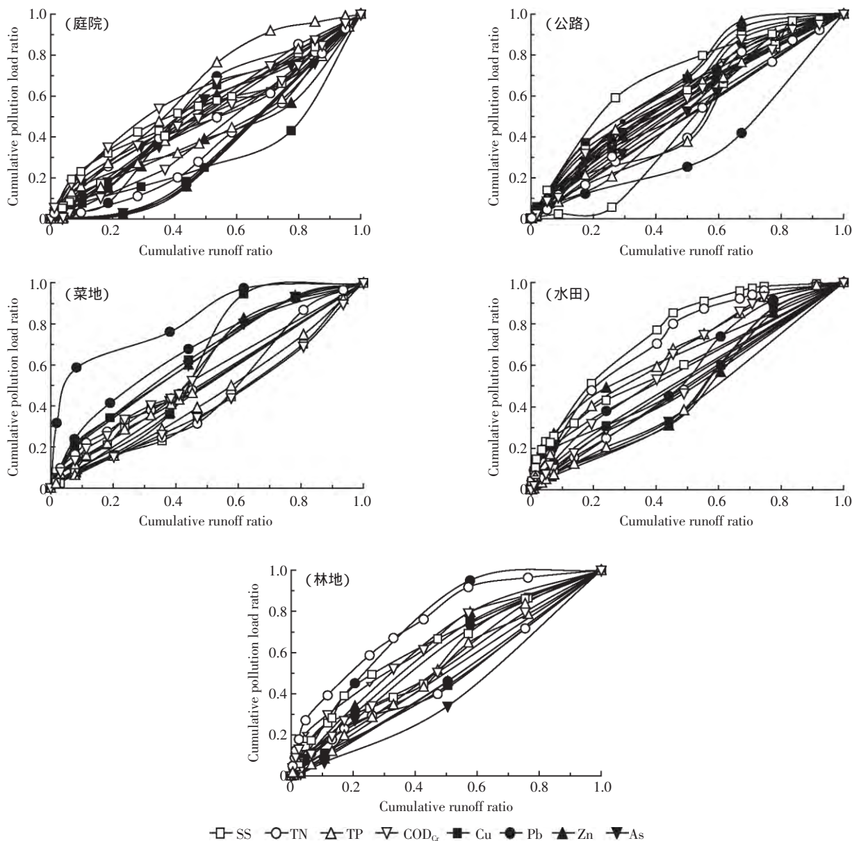
图1 不同用地类型径流场降雨径流初期冲刷 M(V)曲线 Figure 1 M(V) curves of first flush effect in different runoff plots
