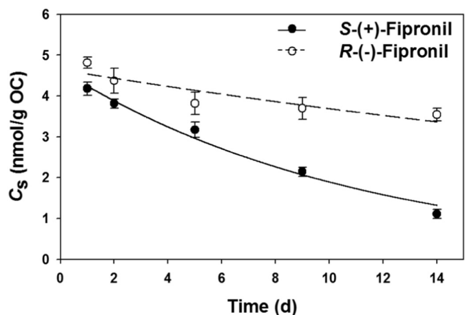
Fig. 2. Stereoselective degradation process of fipronil enantiomers in sediment. Simulative equations for S-(+)- and R(-)-fipronil are C_{S-(+)-fipronil} = 4.64 \times e^{-0.090 \cdot t} (solid circle and real line) and C_{R(-)-fipronil} = 4.64 \times e^{-0.023 \cdot t} (hollow circle and dashed line), respectively. Error bars represent standard deviations of three replicates.
