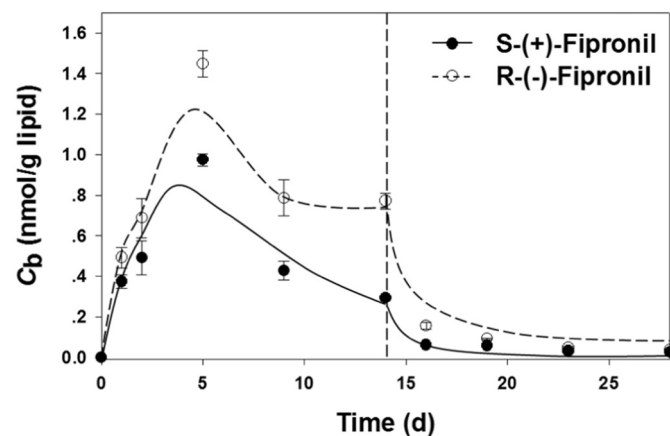
Fig. 3. Toxicokinetic process of fipronil enantiomers in Lumbriculus variegatus . Real and dashed lines are simulative curves for S -(+)-fipronil and R -(-)-fipronil, respectively. Error bars represent standard deviations of three replicates.
